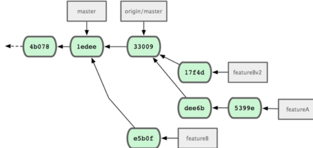
Figure 5.18: Commit history after featureBv2 work
