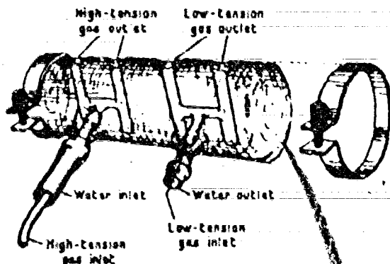
Fig. 6—Chamber for simultaneous equilibration of micro-samples in duplicate of two different carbon-dioxide tensions.
