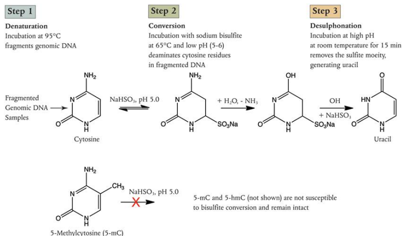
Figure 2: Bisulfite conversion ( www.neb.com )
